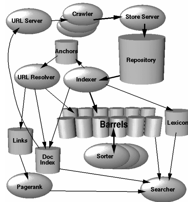
Figure 1. Anatomy of a large scale web search engine, [2]
